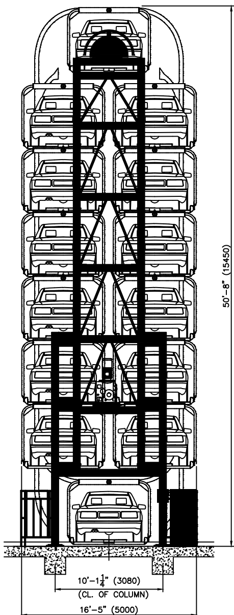
FRONT VIEW
