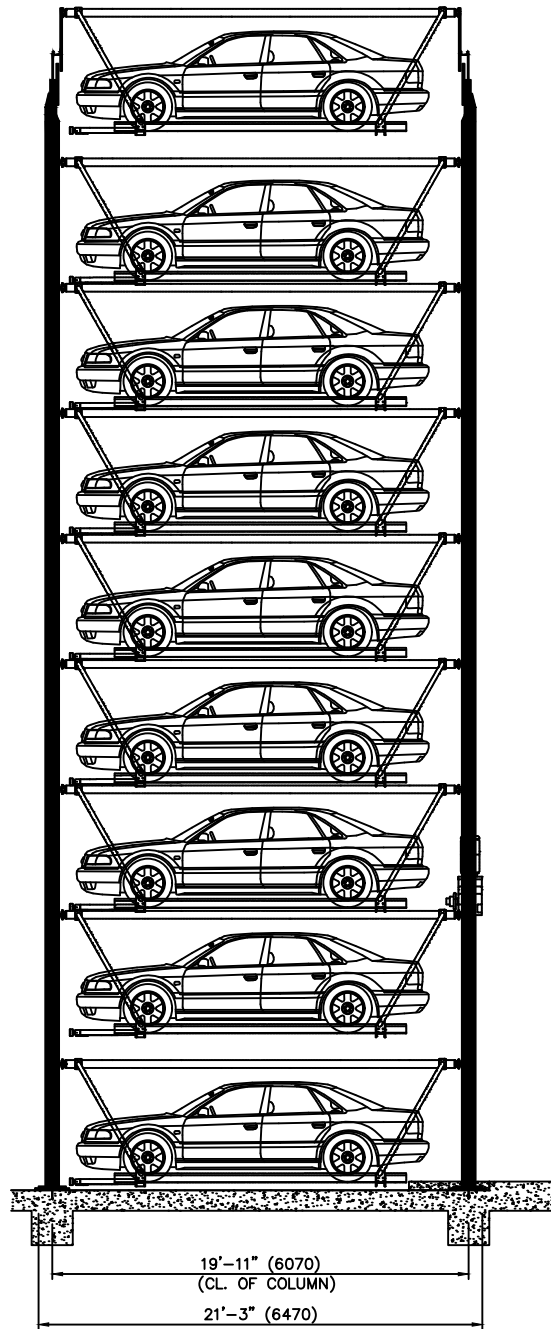
SIDE ELEVATION
