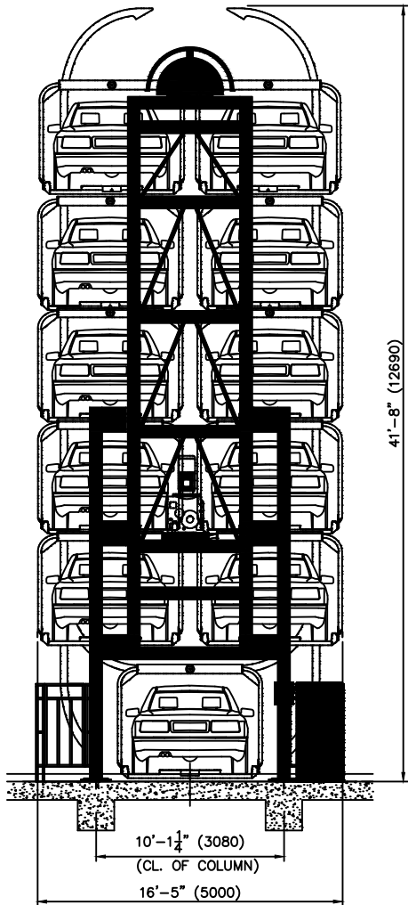
FRONT VIEW
