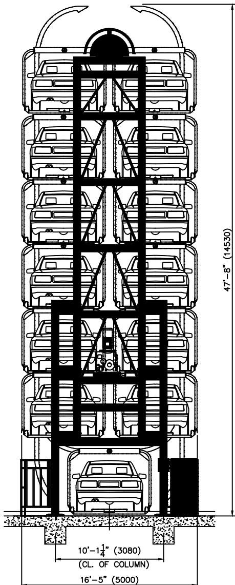
FRONT VIEW
