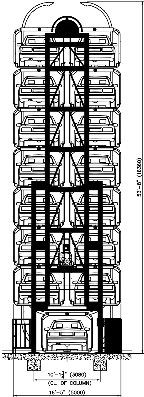
FRONT VIEW
