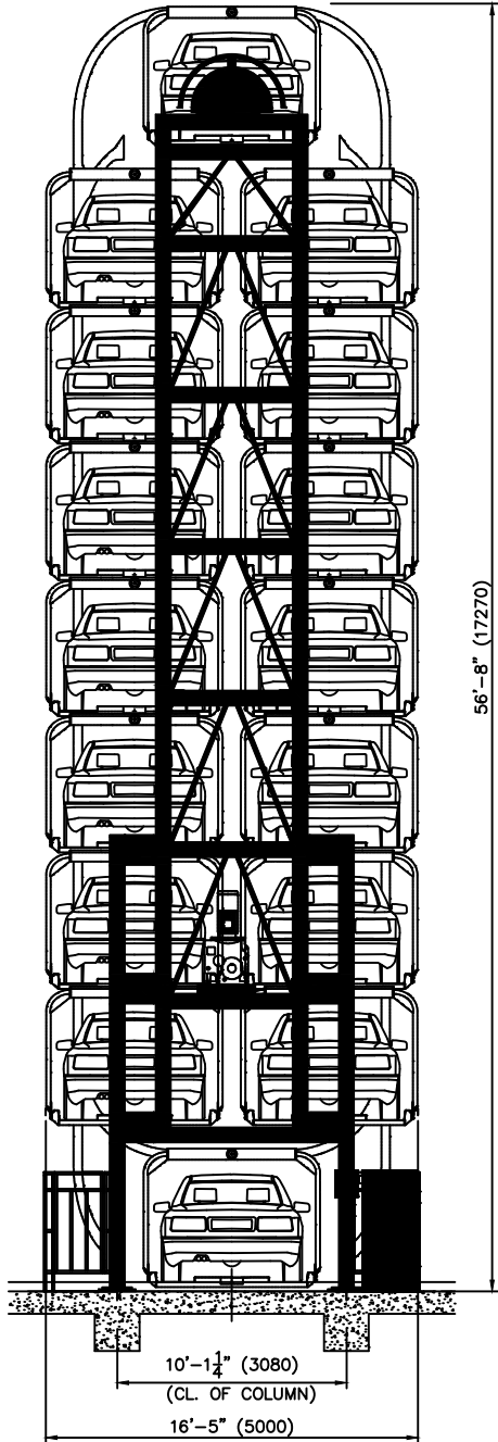
FRONT VIEW
