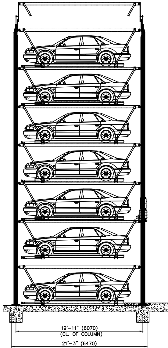
SIDE ELEVATION
